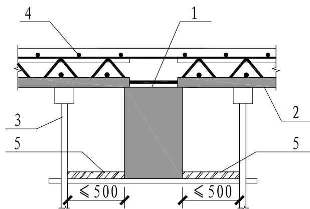
(a) 混凝土梁
